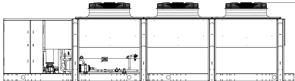
VISTA FRONTAL
